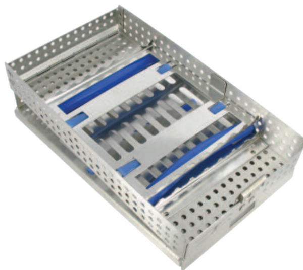
7502D CASSETTE DOUBLE HINGE 16 HOLD DOUBLE RACK 114x203x31mm
