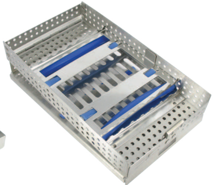
7502D CASSETTE DOUBLE HINGE 16 HOLD DOUBLE RACK 114x203x31mm
